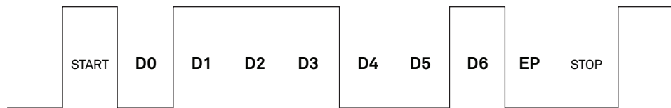
Figure 4 Example SDI-12 transmission of the character 1 (0x31s)
