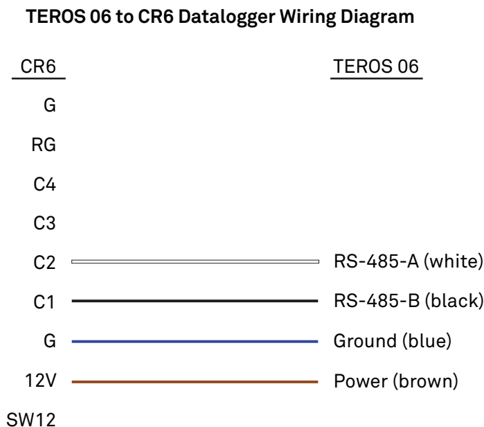
Figure 13 RS-485 interface
