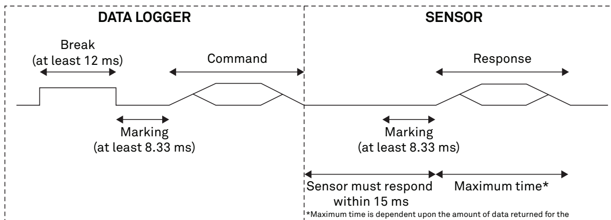
Figure 9 Example data logger and sensor communication
