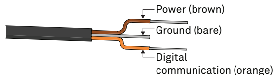
Figure 3 Pigtail cable
