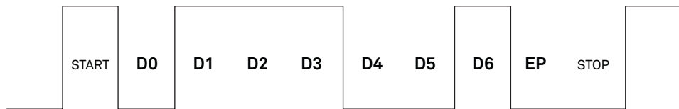
Figure 4 Example SDI-12 transmission of the character 1 (0x31s)
