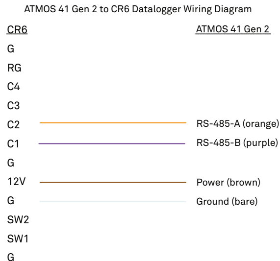
Figure 11 RS-485 interface
