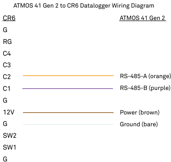
Figure 11 RS-485 interface
